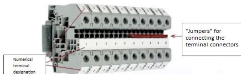
Photo. 6. A method of marking terminal connectors.
