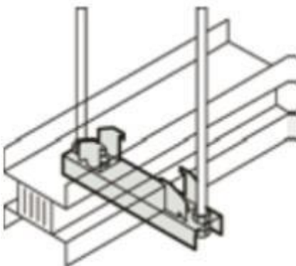
Fig. 21. Installation of busbar to the ceiling
